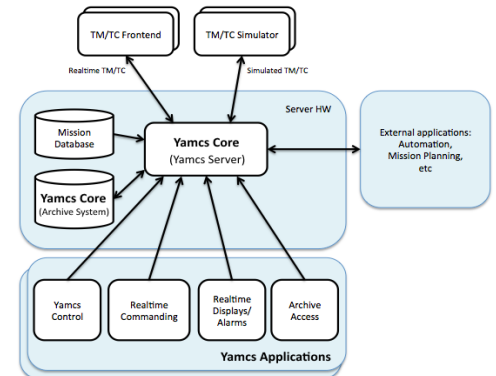
Figure 1 Yamcs component diagram
