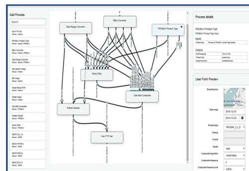
Figure 2 Graphical Workflow Editor
